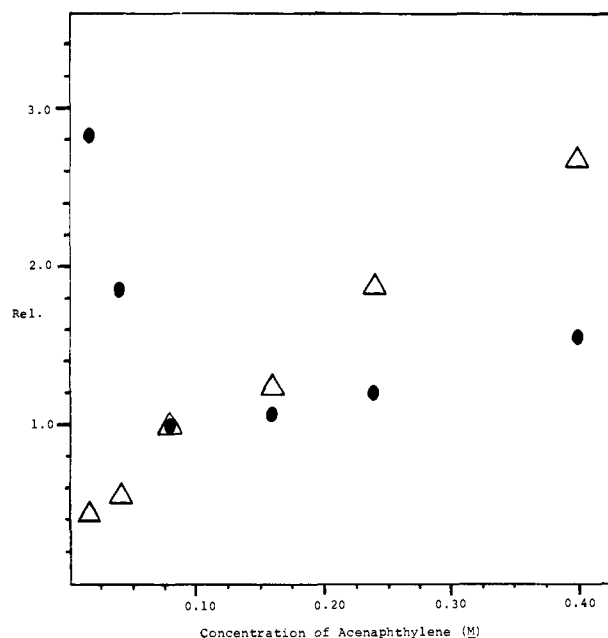
Figure 2. \Phi_{\text{rel}} vs. concentration of acenaphthylene at 35 °C (●) and 55 °C (Δ). \Phi_{\text{rel}} is defined as the ratio of the dimerization quantum efficiency at a given initial concentration of acenaphthylene divided by the quantum efficiency for an initial concentration of 0.08 M acenaphthylene at a given temperature. Each point is the average of at least duplicate measurements.
